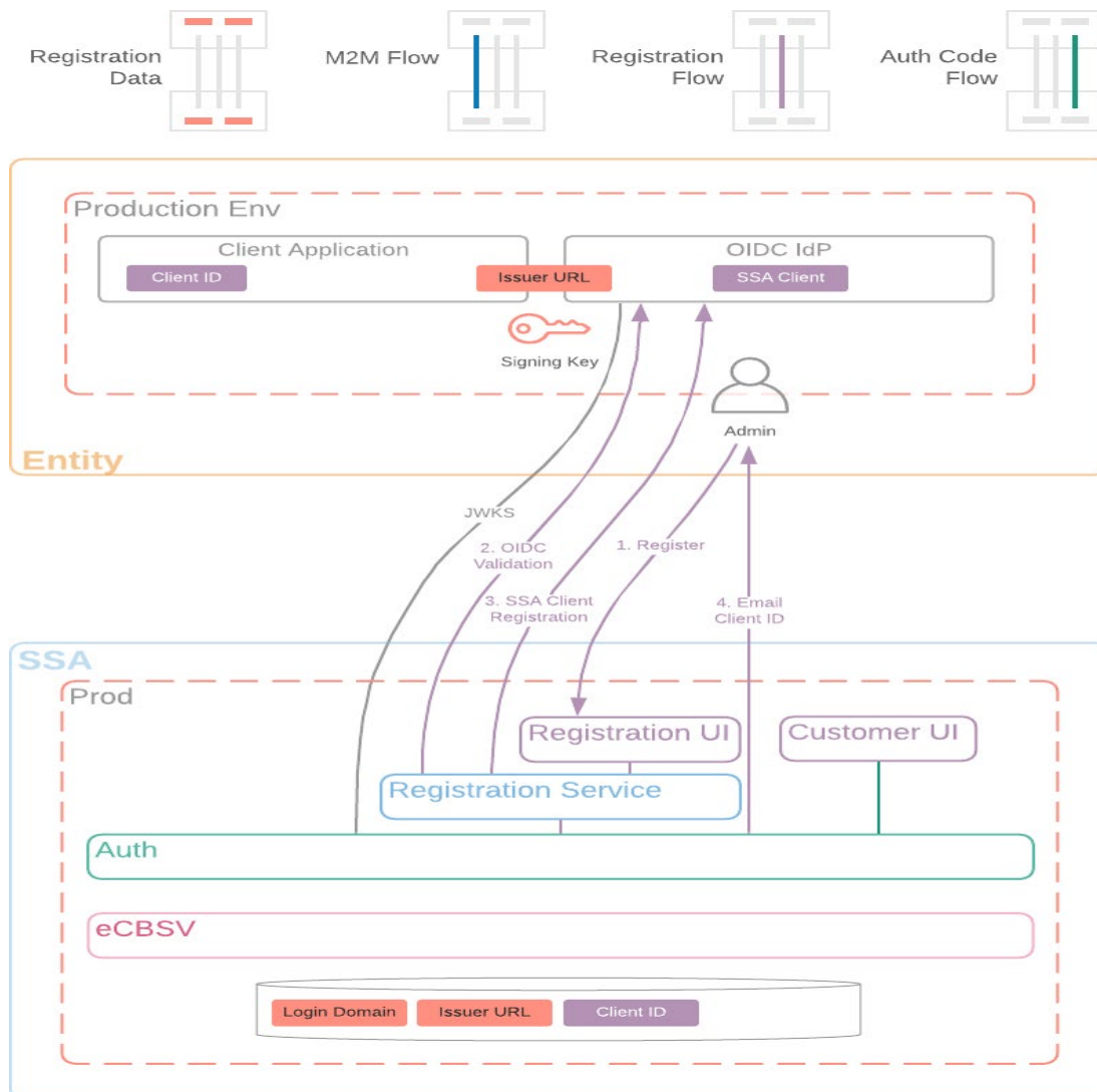
Figure 1.2 - Registration Flow
